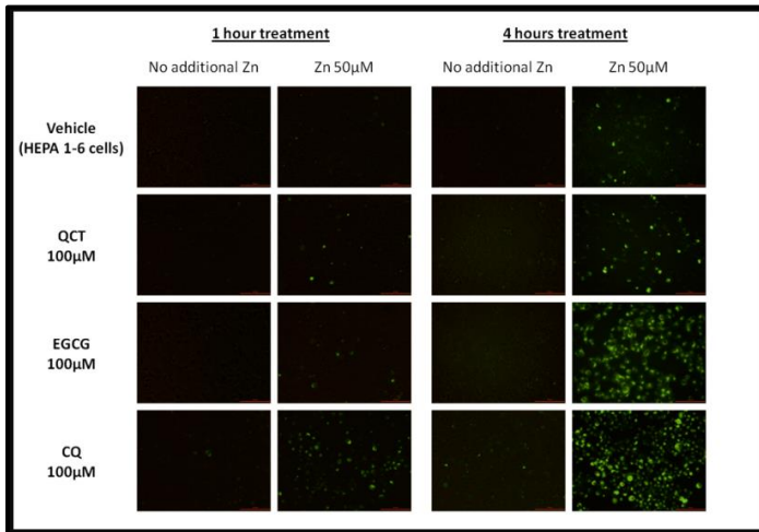
These 2 Charts Shows EGCG Is Even More Effective a Zinc Ionophore Than Quercetin. (CQ is Clloquinol; HCQ is Hydroxychloroquine.) https://pubmed.ncbi.nlm.nih.gov/25050823/ EGCG & Quercetin are effective zinc ionophores. https://pubmed.ncbi.nlm.nih.gov/33732940/ Clloquinol (above) inhibits Covid.
