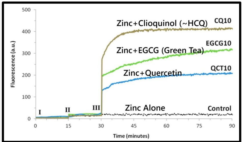
These 2 Charts Shows EGCG Is Even More Effective a Zinc Ionophore Than Quercetin. (CQ is Clloquinol; HCQ is Hydroxychloroquine.) https://pubmed.ncbi.nlm.nih.gov/25050823/ EGCG & Quercetin are effective zinc ionophores. https://pubmed.ncbi.nlm.nih.gov/33732940/ Clloquinol (above) inhibits Covid.
